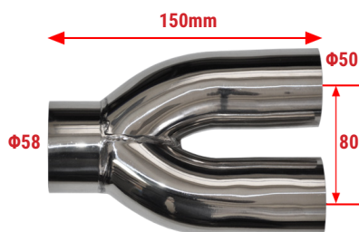
Y-5850 Y-Pipe Length=150mm INΦ=58 OUTΦ=50 S/Steel Y-pipe Suitable for custom made tailpipes 2x76mm
