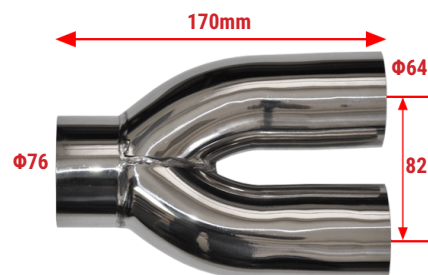
Y-7664 Y-Pipe Length=170mm INΦ=76 OUTΦ=64 S/Steel Y-pipe
