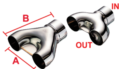
08T-066S A=70 B=108 IN=Φ54 OUT=2xΦ50 08T-087S A=90 B=108 IN=Φ54 OUT=2xΦ54 08T-095S A=100 B=108 IN=Φ54 OUT=2xΦ54 S/Steel Y-pipe
