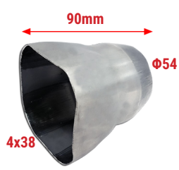
WRX-38 4-1 S/Steel connector Fits on 4 pipes Φ38 each
