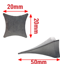
254083 S/Steel Casting Taper for 4-1 pipe connectors
