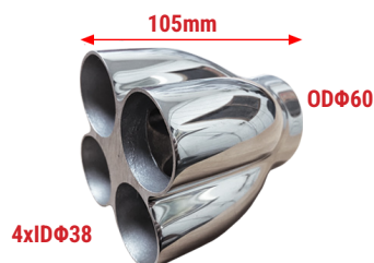
270098P 4-1 Casting S/S connector Fits on 4 pipes Φ38
