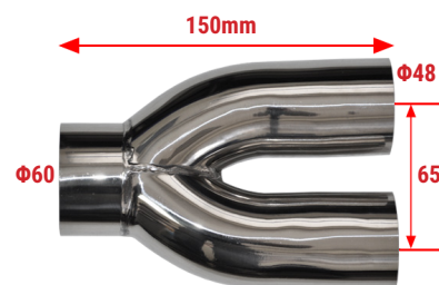
Y-6048 Y-Pipe Length = 150mm INΦ=60 OUTΦ=48 S/Steel Y-pipe
