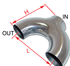
Y3 L=137 INΦ=64 OUTΦ=54 H110
