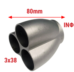
270131 3x38 IN50(OD) 270149 3x38 IN60(OD) 3-1 S/S Casting connector Fits on 3 pipes Φ38 each
