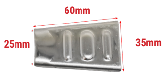
254141 Thickness: 1.4mm Material: S/Steel SUS304
