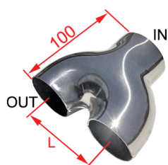
Y1 L=80 INΦ=58 OUTΦ=52
