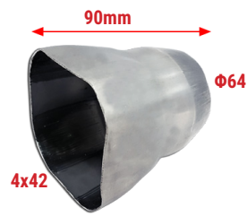
WRX-42 4-1 S/Steel connector Fits on 4 pipes Φ42 each
