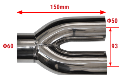
Y-6050 Y-Pipe Length=150 INΦ=60 OUTΦ=50 S/Steel Y-pipe Suitable for custom made tailpipes 2x89mm
