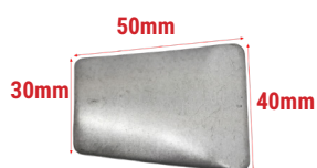
254018 Thickness: 2.0mm Material: Galvanized
