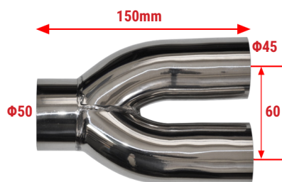
Y-5045 Y-Pipe Length = 150mm INΦ=50 OUTΦ=45 S/Steel Y-pipe
