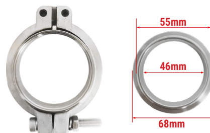
TB5-2 Clamp & Flange for External Waste Gate JB050
