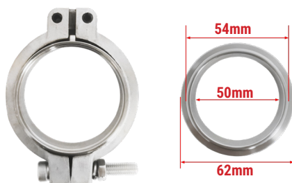
TB5-1 Clamp & Flange for External Waste Gate JB050
