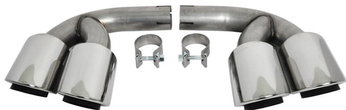
TR-3699 Left & Right S/Steel 304 / Mirror Polished Slant Cut & Side Slant Cut Porsche Cayenne 9YA Turbo '17- Total Length= 370mm Outlet Diameter= 2x100mm Inlet(ID)= 60mm
