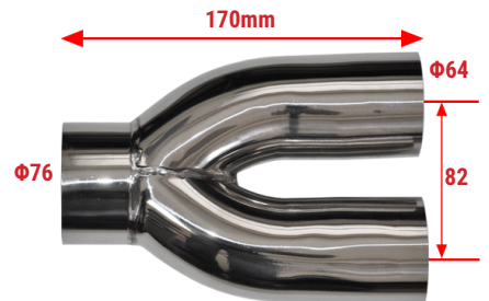
Y-7664 Y-Pipe Length=170mm INΦ=76 OUTΦ=64 S/Steel Y-pipe
