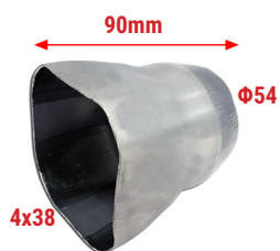
WRX-38 4-1 S/Steel connector Fits on 4 pipes Φ38 each
