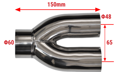
Y-6048 Y-Pipe Length = 150mm INΦ=60 OUTΦ=48 S/Steel Y-pipe
