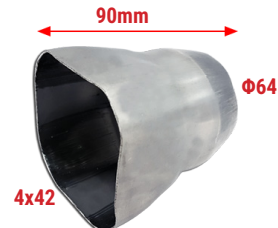
WRX-42 4-1 S/Steel connector Fits on 4 pipes Φ42 each
