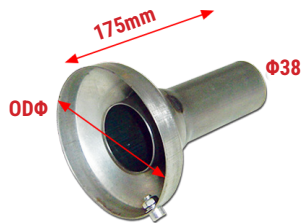
TD89 ODΦ89mm TD101 ODΦ101mm TD115 ODΦ115mm S/Steel DB Killer
