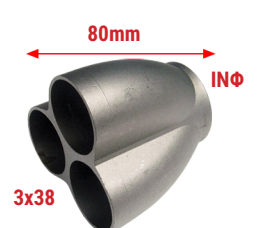
270131 3x38 IN50(OD) 270149 3x38 IN60(OD) 3-1 S/S Casting connector Fits on 3 pipes Φ38 each
