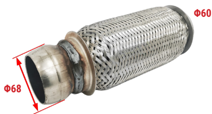
FS45ILOK Repair Flexible for Mercedes Spinter Total Length= 245mm Inlet Diameter(ID)= \Phi 60mm Head Diameter(OD)= \Phi 68mm
