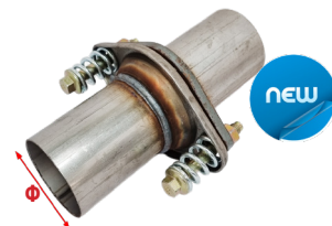
FLEX-50 Length= 200mm Diameter(OD)= \Phi 50mm FLEX-55 Length= 200mm Diameter(OD)= \Phi 55mm FLEX-65 Length= 200mm Diameter(OD)= \Phi 65mm FLEX-80 Length= 200mm Diameter(OD)= \Phi 80mm Universal Flex Spring Joint KIT Material: SUS409
