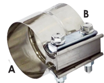
H11700 A=ID \Phi 81mm - B=ID \Phi 76mm H11719 A=ID \Phi 94mm - B=ID \Phi 89mm H11698 A=ID \Phi 105mm - B=ID \Phi 100mm H11688 A=ID \Phi 115mm - B=ID \Phi 110mm H11683 A=ID \Phi 119mm - B=ID \Phi 114mm H11678 A=ID \Phi 132mm - B=ID \Phi 128mm H11675 A=ID \Phi 125mm - B=ID \Phi 120mm H11639 A=ID \Phi 158mm - B=ID \Phi 152mm
