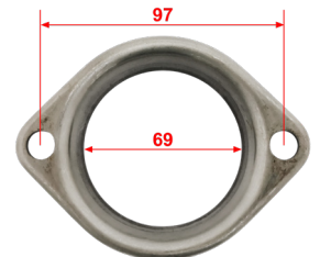
210086 S/Steel BMW M6 E63 T:2.5
