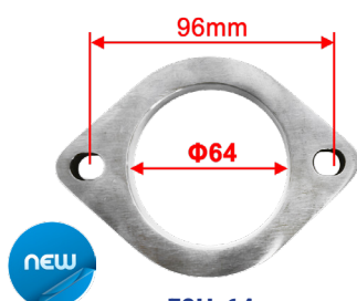
F2H-64 S/Steel Thickness: 10mm
