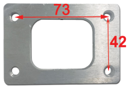
FL-T25 S/Steel For T25-T28-GT25-GT28
