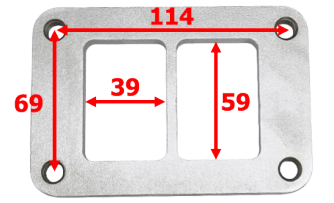
FL-T6 S/Steel For T6
