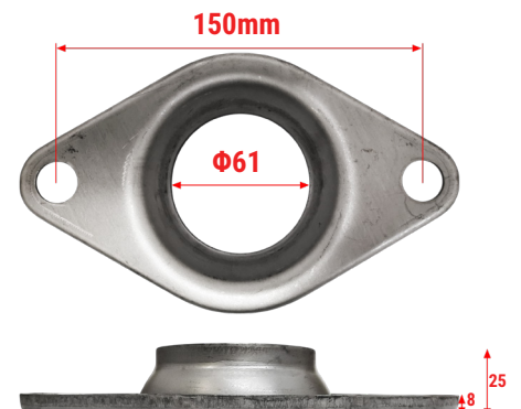
FL-PRIUS S/Steel Toyota Prius
