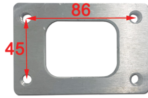
FL-T3 Chromed For T3
