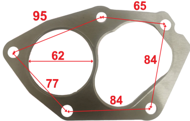
G-EVO S/Steel Fits Mitsubishi EVO 4-9
