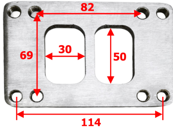
FLT6-T4 S/Steel From T6 to T4
