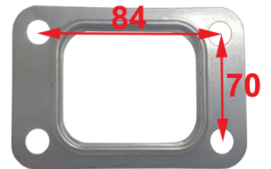
G-T66 S/Steel Fits FL-T4
