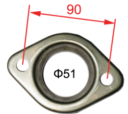
211035-01S S/Steel Honda Civic VTec
