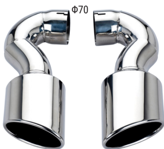
BL224-TDi Left & Right S/Steel 304 Fits ALL TDi models from 02-10 VW Touareg 3.6i VR6 (280Hp) 07-Up VW Touareg 4.2i V8 (310Hp) 04-Up Oval= 152x95mm Inlet(ID)= 70mm
