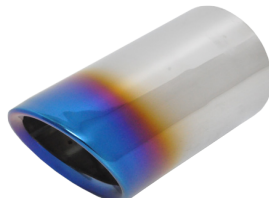
A044 Silver B044 Blue (Burned) M044 Black S/Steel 304 / Slant Cut VW Golf/Passat, AUDI Total Length = 150mm Outlet Dimensions = 76mm Inlet(ID)= \Phi 64 mm With Special clips which lock on the OEM tailpipes No welding needed
