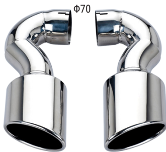
151602-TDi Left & Right S/Steel 304 Fits ALL TDi models from 02-10 VW Touareg 3.6i VR6 (280Hp) 07-Up VW Touareg 4.2i V8 (310Hp) 04-Up Oval= 119x81mm Inlet(ID)= 70mm
