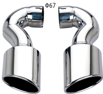
151602-C Left & Right S/Steel 304 VW Touareg 3.2i VR6 03-Up Oval= 119x81mm Inlet(ID)= 67mm
