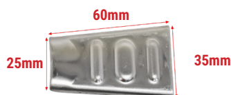
254141 Thickness: 1.4mm Material: S/Steel SUS304
