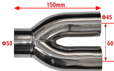
Y-5045 Y-Pipe Length = 150mm INΦ=50 OUTΦ=45 S/Steel Y-pipe
