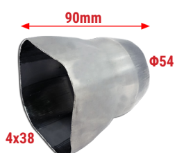
WRX-38 4-1 S/Steel connector Fits on 4 pipes Φ38 each
