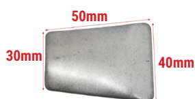
254018 Thickness: 2.0mm Material: Galvanized
