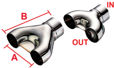
08T-066S A=70 B=108 IN=Φ54 OUT=2xΦ50 08T-087S A=90 B=108 IN=Φ54 OUT=2xΦ54 08T-095S A=100 B=108 IN=Φ54 OUT=2xΦ54 S/Steel Y-pipe
