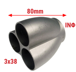
270131 3x38 IN50(OD) 270149 3x38 IN60(OD) 3-1 S/S Casting connector Fits on 3 pipes Φ38 each
