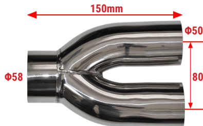
Y-5850 Y-Pipe Length=150mm INΦ=58 OUTΦ=50 S/Steel Y-pipe Suitable for custom made tailpipes 2x76mm
