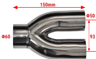
Y-6050 Y-Pipe Length=150 INΦ=60 OUTΦ=50 S/Steel Y-pipe Suitable for custom made tailpipes 2x89mm
