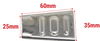
254141 Thickness: 2.0mm Material: S/Steel SUS304
