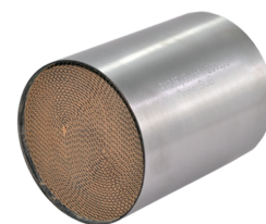
SUB43 Diameter= 130mm Length= 130mm Euro4 / 200cpsi (Cells) High Loading / Premium Quality
