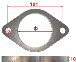
FL7-50 \Phi = 50mm FL7-54 \Phi = 54mm FL7-60 \Phi = 60mm FL7-64 \Phi = 64mm Mild Steel
