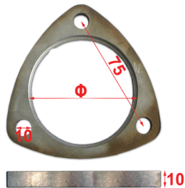
FL22-48 \Phi =48mm FL22-50 \Phi =50mm FL22-54 \Phi =54mm FL22-60 \Phi =60mm FL22-64 \Phi =64mm Mild Steel
