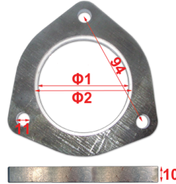
FLT-70 \Phi 1=67, \Phi 2=70 FLT-76 \Phi 1=73, \Phi 2=76 Mild Steel
