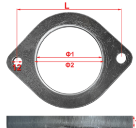
FL8012 \Phi 1=77, \Phi 2=80, L120 FL9012 \Phi 1=87, \Phi 2=90, L120 FL10112 \Phi 1=98, \Phi 2=101, L130 Mild Steel
