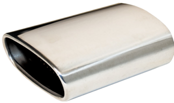
BL172 S/Steel 304 Slant Cut / Double Layer Total Length= 210mm Outlet Dimensions= 152x78mm Inlet(OD)= 152x78mm
